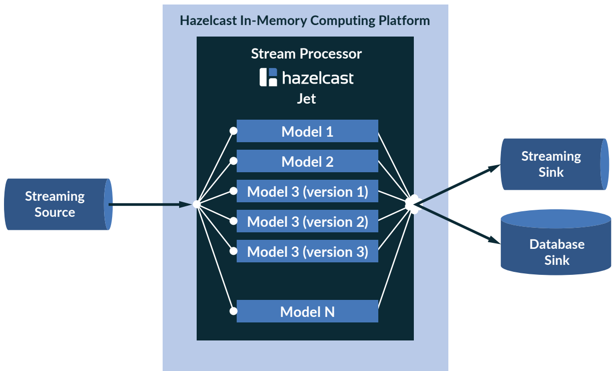
Figure 5. Machine Learning Models in Parallel
